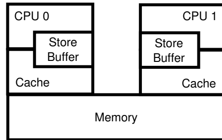
Figure 15.1: System Architecture With Store Buffers
