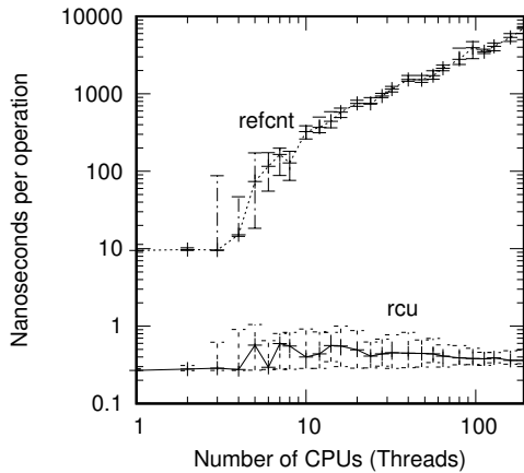
Figure 9.27: Performance of RCU vs. Reference Counting
