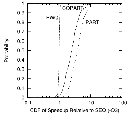
Figure 6.30: Partitioned Coroutines
