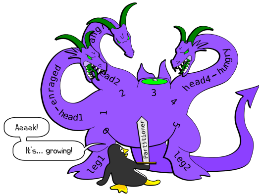
Figure 10.14: Partitioning Problems
