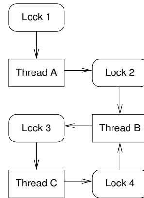
Figure 7.3: Deadlock Cycle
