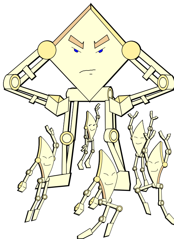
Figure 17.5: Astounding Accelerators
