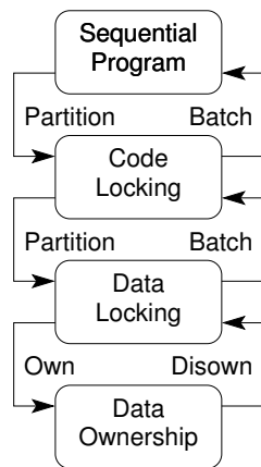
Figure 6.10: Design Patterns and Lock Granularity
