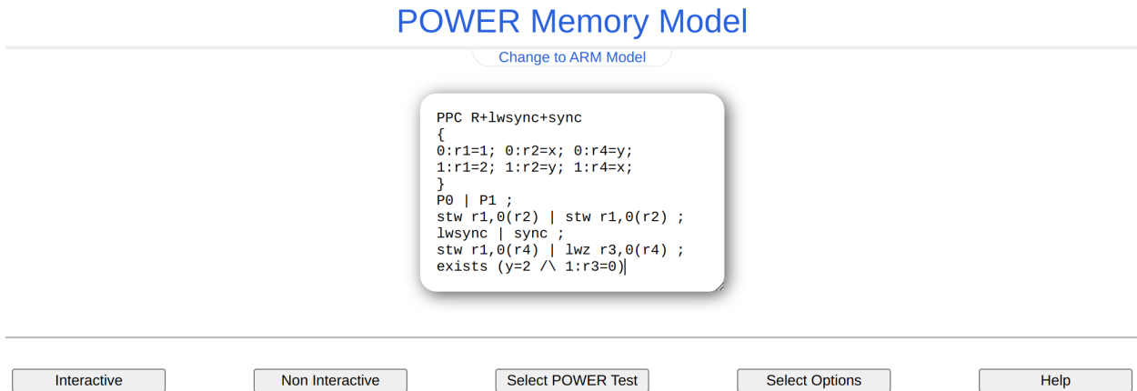
Figure 15.15: PPCMEM Initial R State
