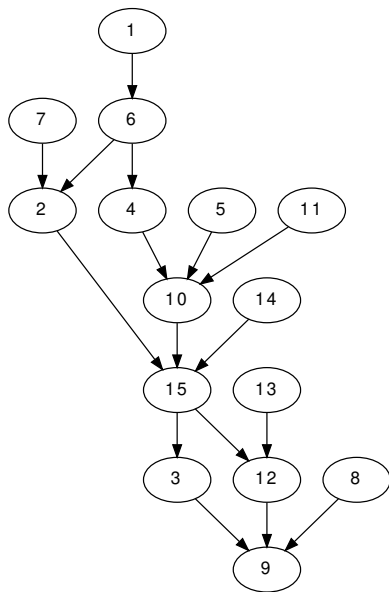
Figure 15.8: Possible Global Orders With More Simultaneous Values
