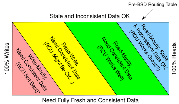
Figure 9.33: RCU Areas of Applicability
