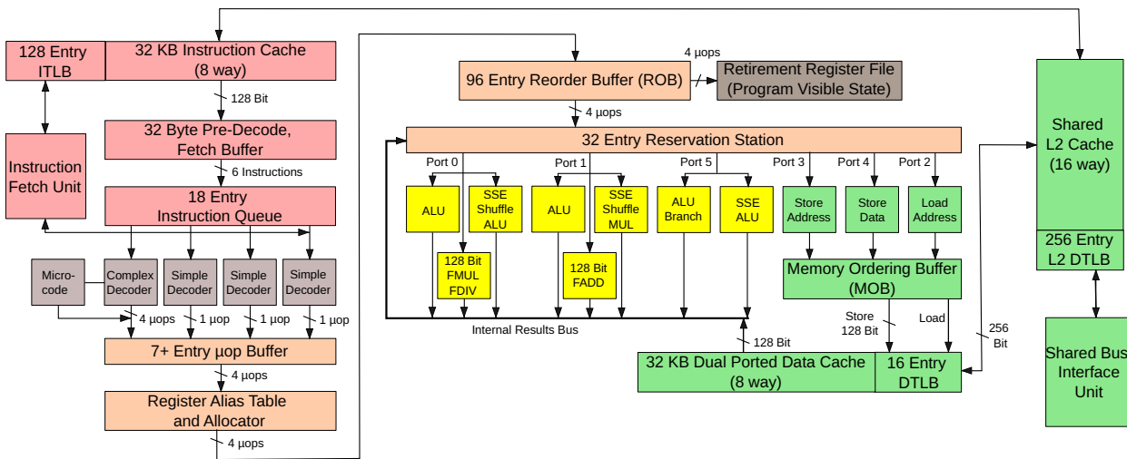
Figure 15.1: Intel Core 2 Architecture
