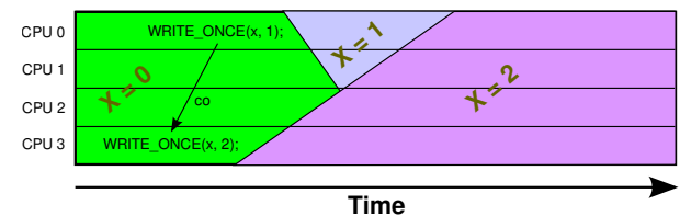
Figure 15.13: Store-to-Store is Counter-Temporal
