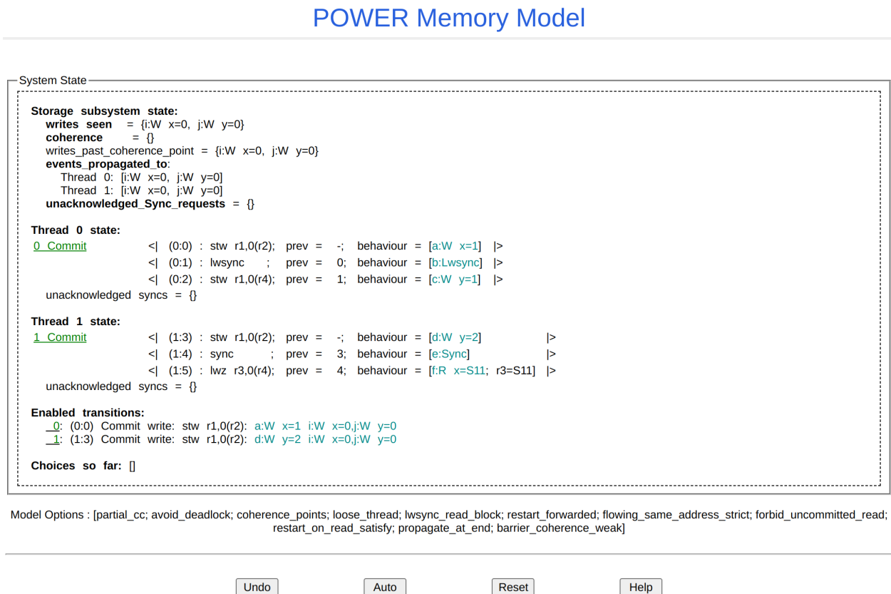
Figure 15.16: PPCMEM First R Step
