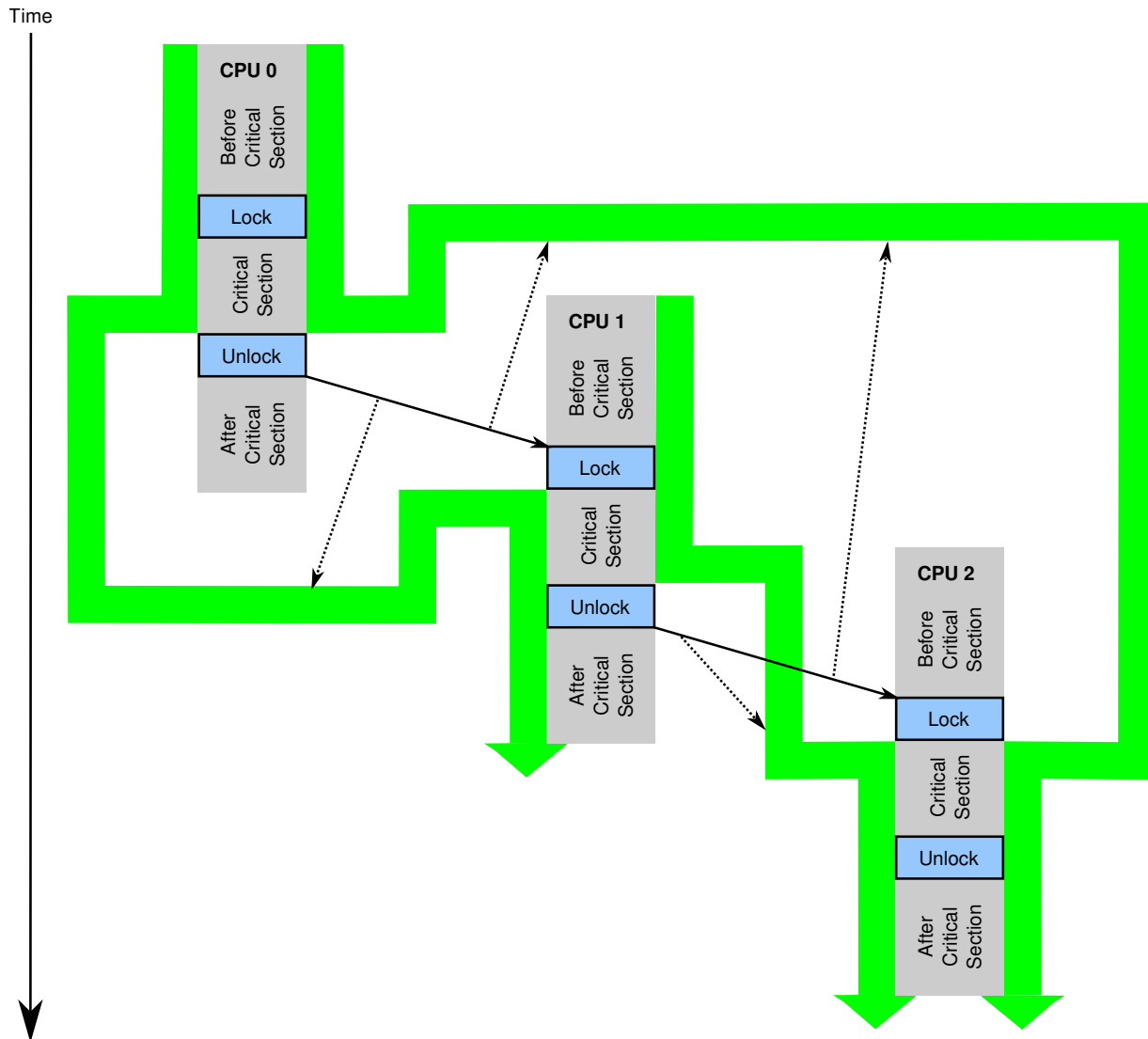
Figure 15.24: Locking Intuitions
