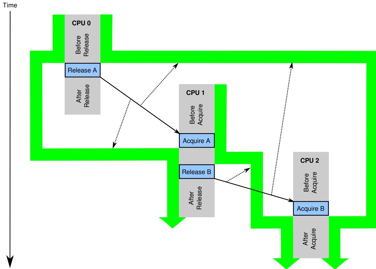
Figure 15.25: Release-Acquire Intuitions
